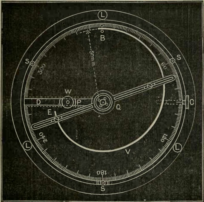
Fig. 18A, Plan of Walker and Barber's Tester.
