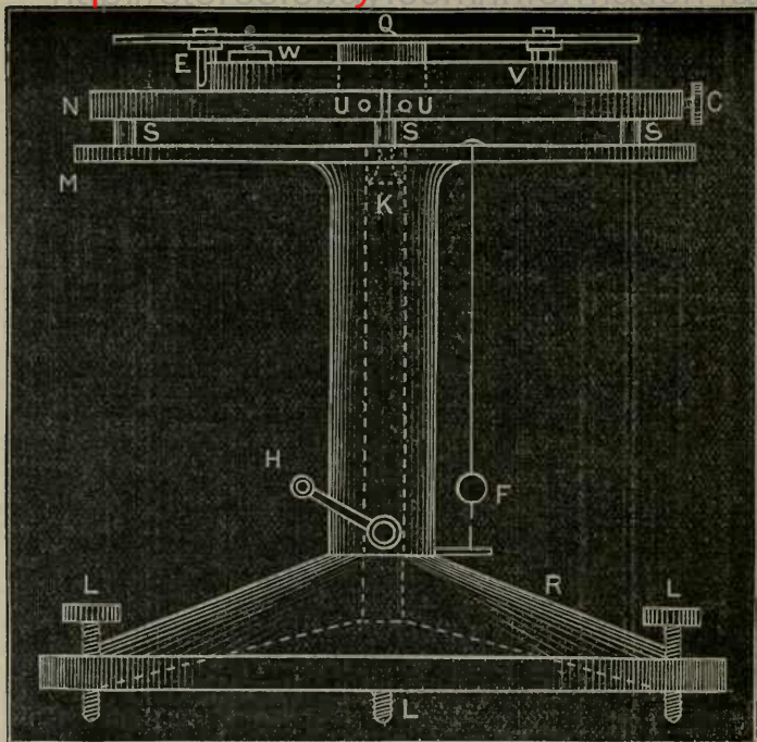
Fig. 18B, Elevation of Walker and Barber's Tester.
