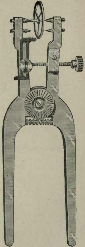
Fig. 50. Plyer-shaped Poising Callipers.
