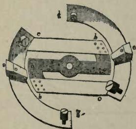
Fig. 30.—Hartnup's balance.
