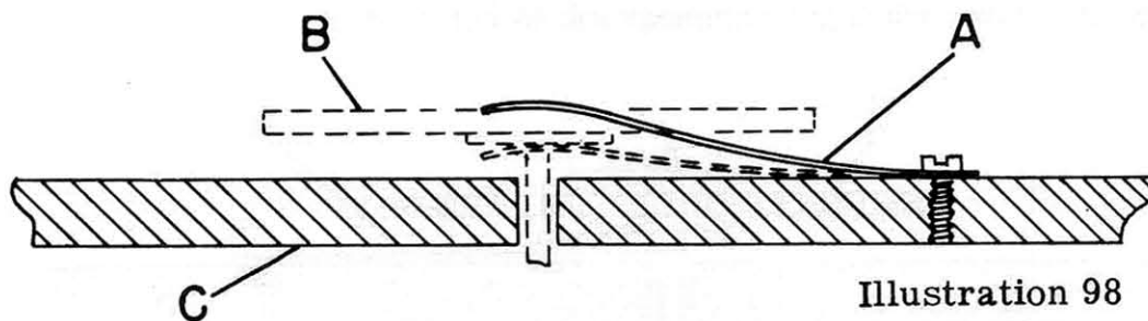
A - Seconds wheel tension spring C - Plate
