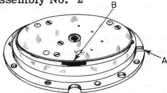
Lower Rotor Plate and Automatic Winding Mechanism
