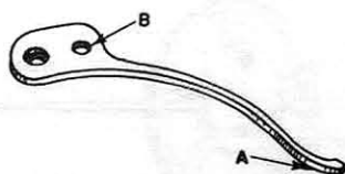
Chronograph Pivoted Detent Spring Assembly No. 13
