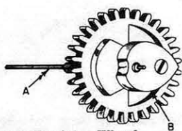
Minute Register Wheel Assembly No. 24
