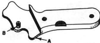
Hour Flyback Lever Bridge Assembly No. 1
