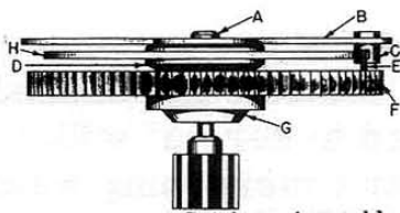
Catch-up Assembly Assembly No. 1
